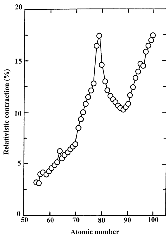
Fig. 2. Calculated relativistic contraction of the 6s level as a function of atomic number Z . The actual size of the 6s electron shell for Pt and Au is some 15% smaller than it would be in the absence of the relativistic effect.
