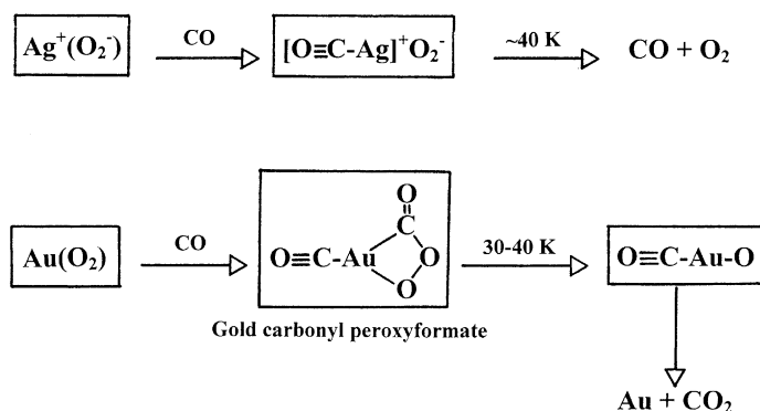
Fig. 3. Reactions of silver and gold oxygen complexes with carbon monoxide in a solid inert gas matrix [15,16].
